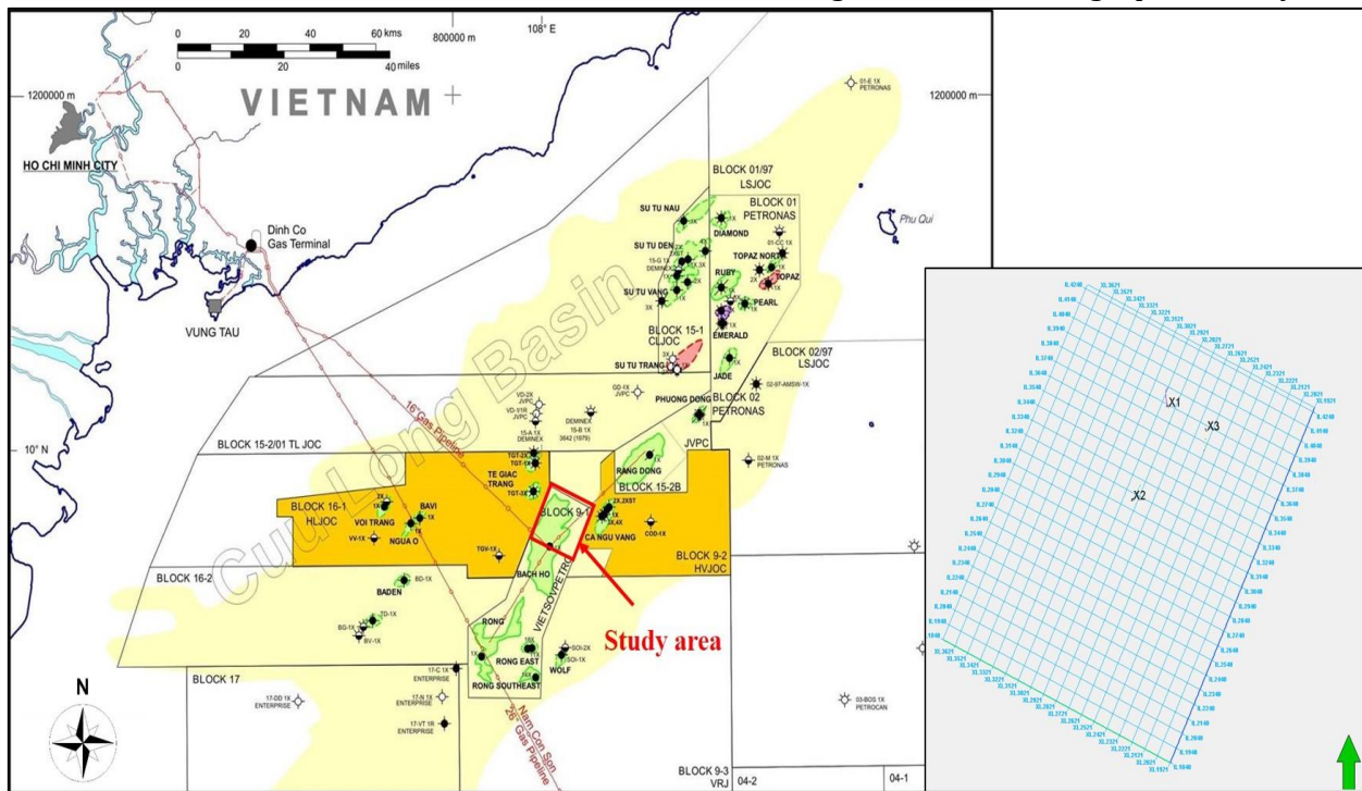
Figure 1. Location map of study area and wells in the seismic survey.
